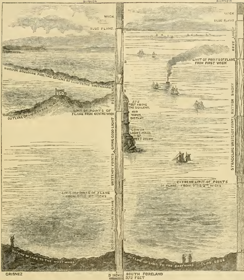
From a tracing on ground glass. The flame from measurement of the Calais flame. The landscape as it appeared in the image formed by one of the revolving lenses. GRISNEZ. June 20th 1860.
